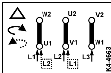
Delta connection
