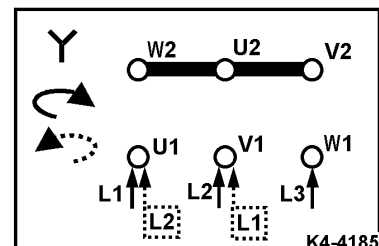
Star connection
